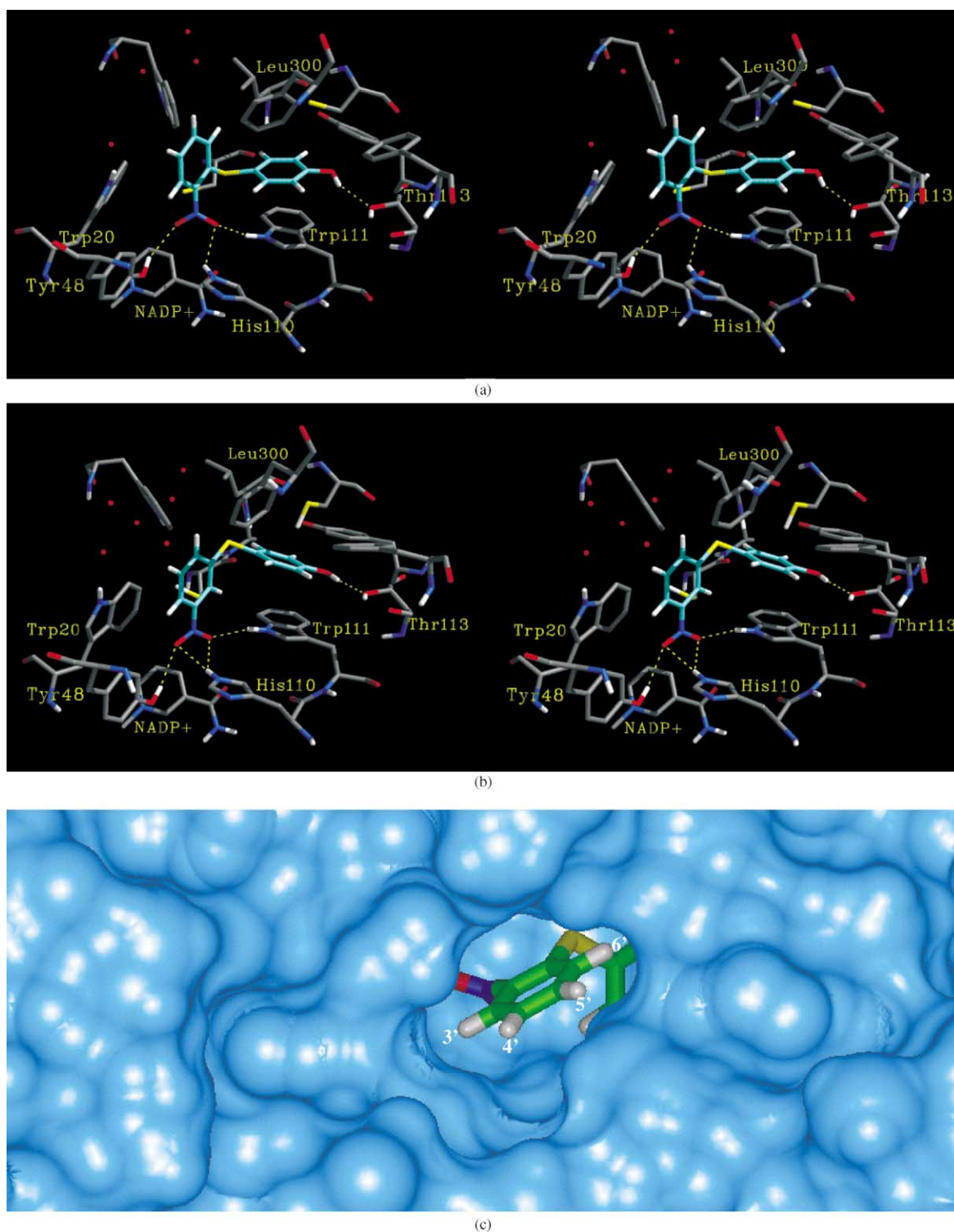
Figure 1. (a) Stereoview of active site residues of ALR2 interacting with the lead inhibitor 4-(2'-nitrophenylmercapto)phenol after refinement with MD. (b) Stereoview of active site residues of ALR2 interacting with the inhibitor 4-(3'-nitrophenylmercapto)phenol after refinement with MD. For clarity, only the polar hydrogens are shown, and hydrogen bonds are shown as dotted lines. Water molecules are shown as dots. (c) Molecular surface of ALR2 with the inhibitor 4-(2'-nitrophenylmercapto)phenol bound at the active site. Positions substituted in the present work are numbered from 3' to 6'.
